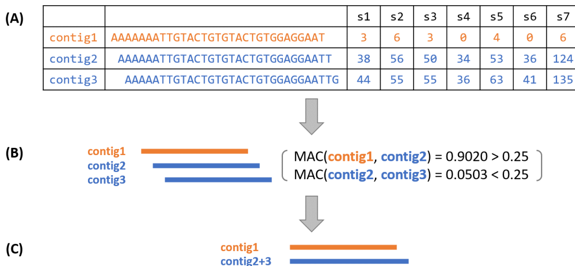
Figure 2: Merging procedure of 3 example contigs: A . Count table of contigs in samples. Both pairs ( contig1 , contig2 ) and ( contig2 , contig3 ) have good overlaps shifting by only one nucleotide, but the sample count vectors of contig1 and contig2 are not compatible. B . Merging intervention considering sample count compatibility between contigs. The mean absolute contrast (MAC) is calculated for each pair, and merging of ( contig1 , contig2 ) is rejected due to a MAC value exceeding threshold. C . The resulting contigs are the initial contig1 and the merged contig from the initial ( contig2 , contig3 ) pair.
