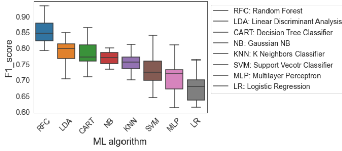
Fig. 10: ML algorithm comparison (no bandwidth limitation)
