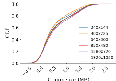
(a) Chunk size per viewport with a 3Mbps bandwidth
