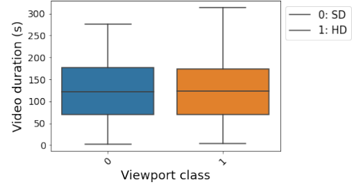
Fig. 11: Video duration distribution (seconds)
