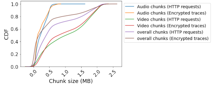
Fig. 3: Chunk size CDF
