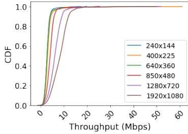
(c) Throughput per viewport for a unlimited bandwidth
