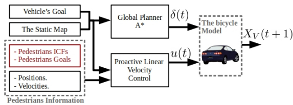
Fig. 4. The Proactive Navigation Policy
