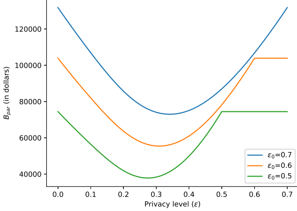
Fig. 4. Variation in the budget for Laplace mechanism \mathcal{L}^1_{\epsilon_0} under privacy at risk considering explicit randomness in the Laplace mechanism for the illustration in Section 5.3.
