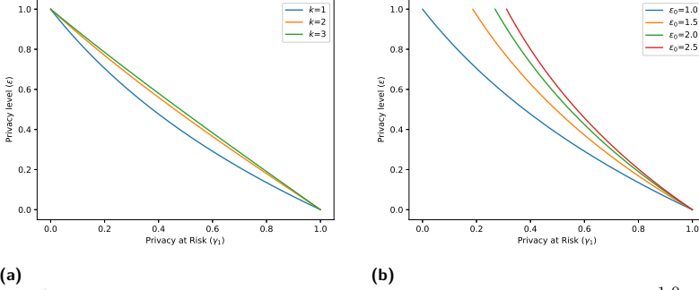
(a) (b) Fig. 1. Privacy level \epsilon for varying privacy at risk \gamma_1 for Laplace mechanism \mathcal{L}_{\epsilon_0}^{1,0} . In Figure 1a, we use \epsilon_0 = 1.0 and different values of k . In Figure 1b, for k = 1 and different values of \epsilon_0 .
