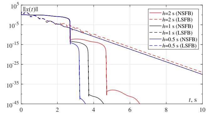
Fig. 2. Comparison of nonlinear (NSFB) and linear state feedback (LSFB) for different time delays
