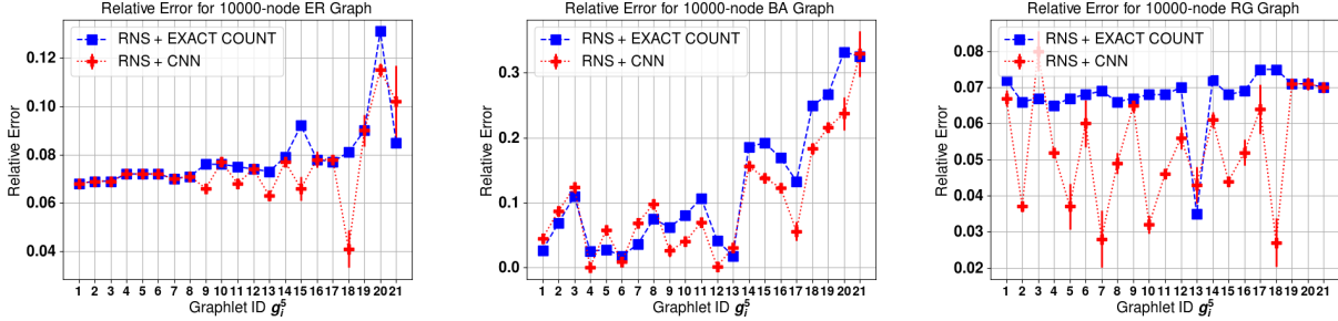
Figure 14: Relative Errors for 5-node Graphlets for Large Random Graphs
