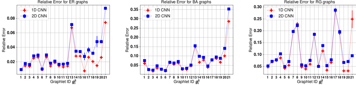
Figure 7: 1-D CNN v.s. 2-D CNN for 5-node graphlets
