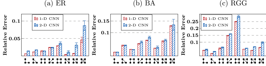
Figure 6: 1-D CNN v.s. 2-D CNN Performance
