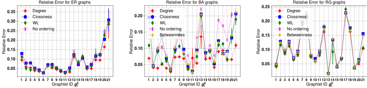
Figure 15: Relative Errors for 5-node Graphlets with Different Node Orderings
