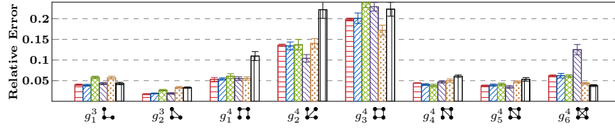
Figure 8: Relative Errors of 1-D CNN and Competing Methods for 4-node graphlets
