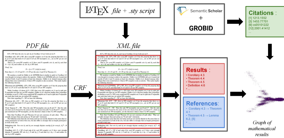
Figure 6: Flow of the algorithm. We convert a PDF file into an XML file using a CRF, or we use source files for this purpose, then we extract results and references. Finally, we associate references with papers in the corpus to build a graph of mathematical results.
