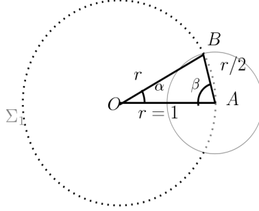
Figure 1: Angle covered by disk of radius 1/2 is = 2\alpha .
