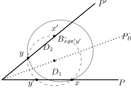
Figure 3: x, y \in \text{Int}_{\mathcal{S}}(\mathcal{Y}) , on different facets F \subset P, F' \subset P'
