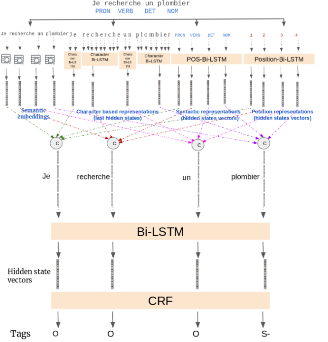
FIGURE 2 – Model architecture (Embeddings Extraction + Main BiLSTM-CRF)
