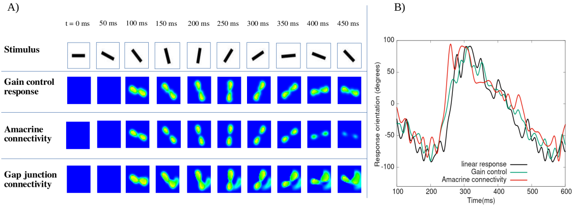
Figure 16: Anticipation for a rotating bar. A) Response to a bar rotating at 4.25\text{rad}/\text{ms} . The first line shows the stimulus, the second line shows the GCells response with gain control, the third line presents the effect of lateral ACells connectivity with w = 0.2\text{ ms}^{-1} , and the last line shows the effect of asymmetric gap junctions with v_{\text{gap}} = 9\text{ mm}/\text{s} . B) Time course response of the bar orientation in the reconstructed retinal representations.
