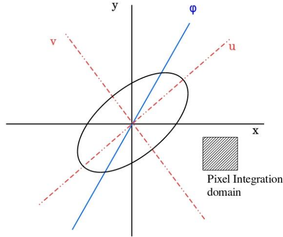
Figure 17: Filter transformation description [33]. The original system of axes is represented by x and y , and the ellipse system of axes by u and v . \phi represents the angle of the second axis of the non-orthogonal basis. The integration domain of a pixel is limited by four lines of equations : x = i\delta , x = (i + 1)\delta , y = j\delta and y = (j + 1)\delta . Rewriting these four equations in the new system of axes through a coordinate change enables us to write the equation (61) .
