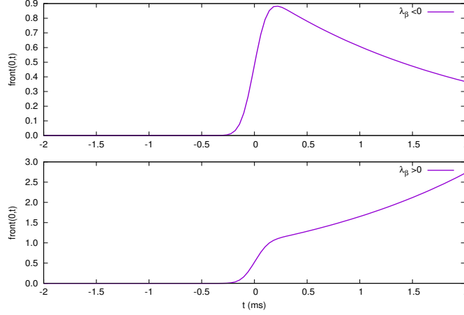
Figure 6: Front (43) for different values of \lambda_\beta (Purple) as a function of time, for the cell \gamma = 0 . All figures are drawn with v = 2 mm/s; \sigma = 0.2 mm. Top. \lambda_\beta = -0.5 ms^{-1} ; Bottom. \lambda_\beta = 0.5 ms^{-1} .
