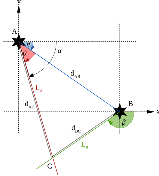
Figure 19: Geometry of connection between 2 neurons. \alpha ( \beta ) is the angle of the neuron A 's branch with length L_A (neuron B 's branch with length L_B ) with respect to the horizontal axis. \theta is the angle between the segment connecting AB and the branch A . C represents the virtual point that lies at the intersection of the branches of length L_A and L_B . d_{AB} (resp. d_{AC} , d_{BC} ) denotes the distance between A and B (resp. A , C and B,C ). Note that d_{AC} \leq L_A , d_{BC} \leq L_B .
