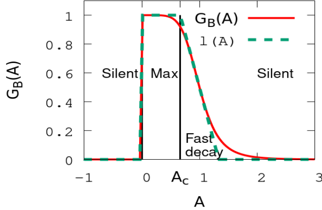
Figure 3: Gain control (9) as a function of activity A . The function l(A) , in dashed line, is a piecewise linear approximation of G_B(A) from which 3 regions are roughly defined. In the region "Silent" the gain vanishes so the cell does not respond to stimuli; in the region "Max", the gain is maximal so that cell behaviour does not show any difference with a not gain-controlled cell; the region "Fast decay" is the one which contributes to anticipation by shifting the peak in the cell's activity (see section 3.1). The value A_c = \frac{2}{3} corresponds to the value of activity where gain control, in the piecewise linear approximation, becomes effective.
