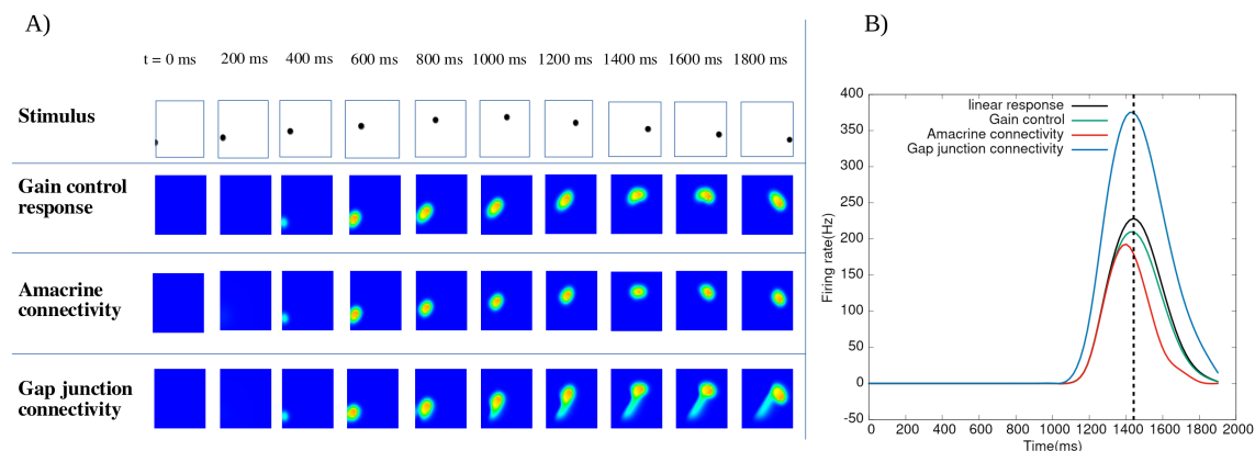
Figure 15: Effect of anticipatory mechanisms on a parabolic trajectory. A) Response to a dot moving along a parabolic trajectory. The first line shows the stimulus, the second line shows the GCells response with gain control, the third line presents the effect of lateral ACells connectivity with w = 0.3 \text{ ms}^{-1} , and the last line shows the effect of asymmetric gap junctions with v_{gap} = 9 \text{ mm/s} . B) Time course response of a cell responding to the dot near the trajectory turning point. Linear response corresponds to the response to the stimulus without gain control.
