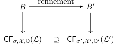
Figure 6: Anti-monotony of the counterfactual builder under refinement of the behavioral model.
