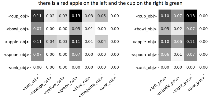
Fig. 8. Output tensor projected onto 2 axis, showing the characteristics associated with objects described in the same sentence as in Figure 7.
