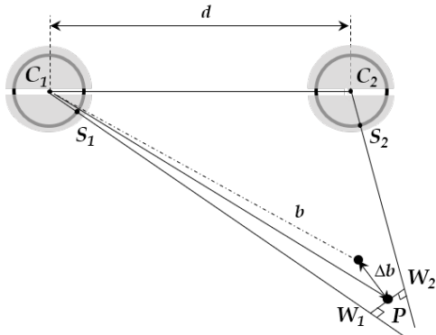
Fig. 6: Illustration of triangulation with two fish-eye cameras.
