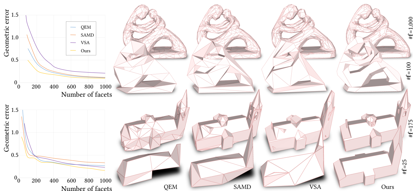
Fig. 18. Comparisons with surface approximation methods. The left curves, that measure the geometric error in function of the number of facets of the output mesh, show that our algorithm outclasses simplification methods for both a freeform object (FERTILITY, top) and a nearly piecewise planar structure (LANS, bottom). QEM [Garland and Heckbert 1997] cannot output large meaningful facets whereas SAMD [Salinas et al. 2015] and VSA [Cohen-Steiner et al. 2004] fail to correct the geometric inaccuracies contained in the dense triangle mesh. For each row, the four meshes contain the same number of facets \#f . The geometric error is measured as the symmetric mean Hausdorff distance between input points and output mesh.
