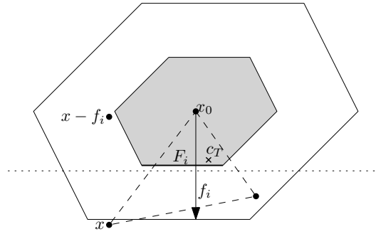
■ Figure 7 A cell (dashed) with a vertex x that is outside of \text{dom}(0, 2\Lambda) . The dotted line is the perpendicular bisector between x and x - f_i .
