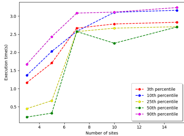
Fig. 5. Execution time by clients number.
