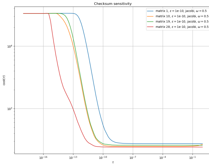
Figure 1.3: Cost function for a given \epsilon , preconditioner, and \omega , but for different matrices.
