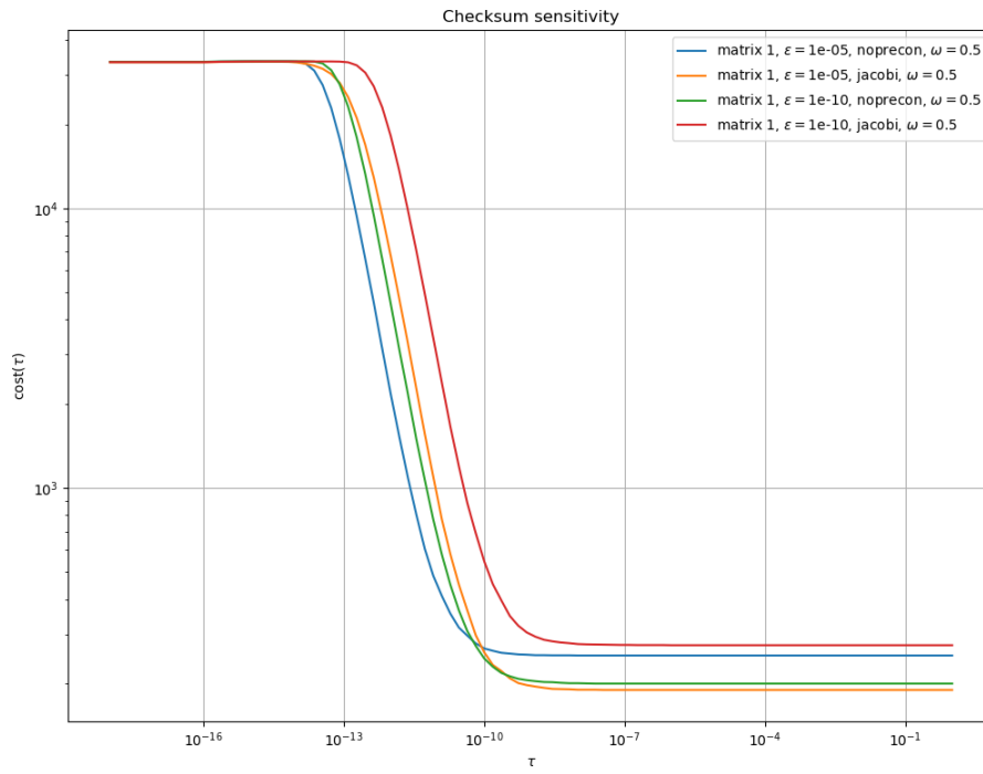
Figure 1.2: Cost function for a given matrix, and \omega , but with different combinations of \epsilon and preconditioner.
