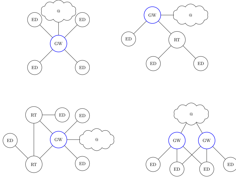
Figure 2: Types of topology: gateway (GW), router (RT) and end device (FD)
