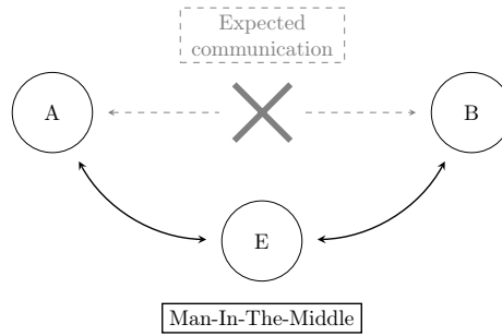
Figure 16: MITM attack.
