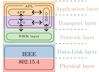
Figure 6: Detail of the Zigbee protocol.
