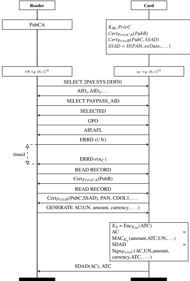
Figure 5: The PayPass-RRP Protocol
