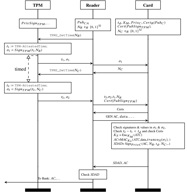
Figure 6: PayCCR [7]: Mastercard’s PayPass-RRP with Collusive-Relay Protection &amp; No Changes to the Issuing Bank
