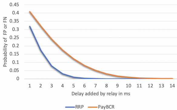
Figure 4: The possible false negative and false positive rates for our implementation of RRP and PayBCR for a range of possible relay speeds
