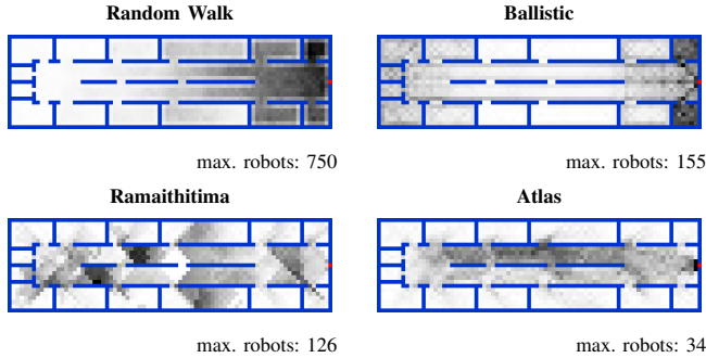
Fig. 6: Heat maps of how often robots have been present on each cell, at the end of a simulation run. Results presented for a 100-robot swarm. The opacity of each cell is mapped to a different scale for each heat map.
