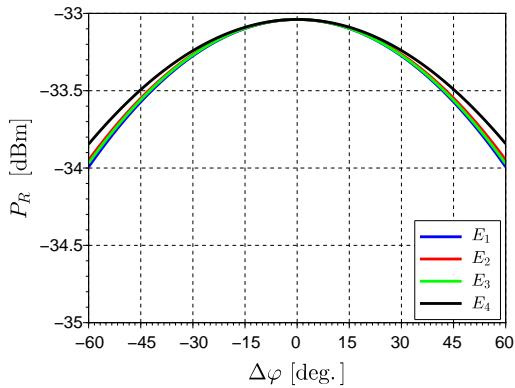
Figure 3. The power level variation with respect to the deviation of the desired phases \varphi_i
