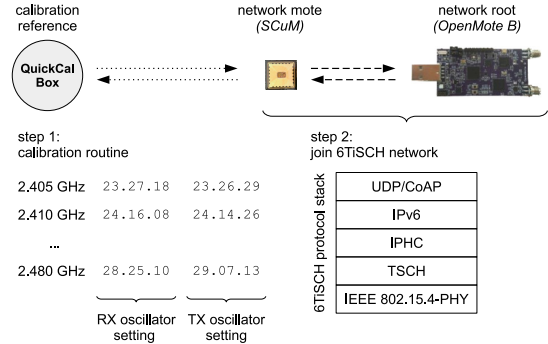
Fig. 5. After quick calibration has finished, SCuM records the frequency settings for both transmitting (TX) and receiving (RX) on each of the 16 frequencies. These settings are represented as X.Y.Z where X, Y and Z each represent the setting of a 5-bit tuning DAC. The firmware then applies these settings while executing the channel-hopping 6TiSCH protocol.
