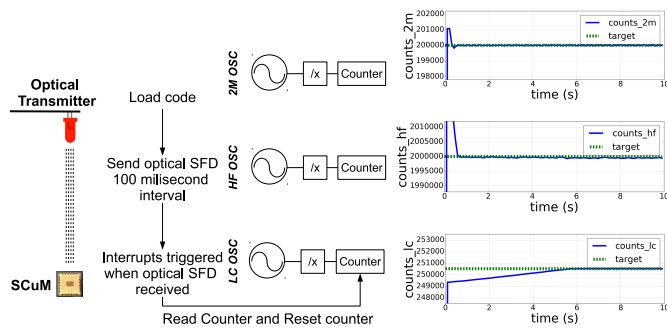
Fig. 2. Optical calibration, using the optical bootloader. After loading the firmware into RAM, the optical bootloader sends 100 pulses, one every 100 ms. The firmware captures and resets the counters of timers attached to the 3 oscillators at each pulse. It then uses that information for calibrating the 2M and HF oscillators.
