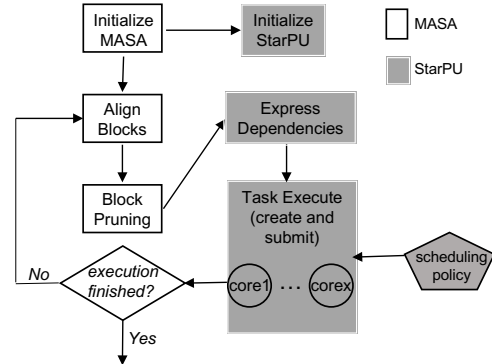
Fig. 6. MASA-StarPU flowchart
