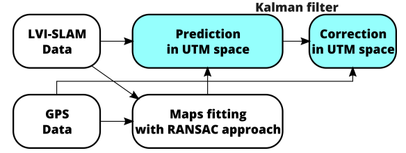
Fig. 5. Scheme of Kalman filter (in blue) used for LVI-GPS fusion.
