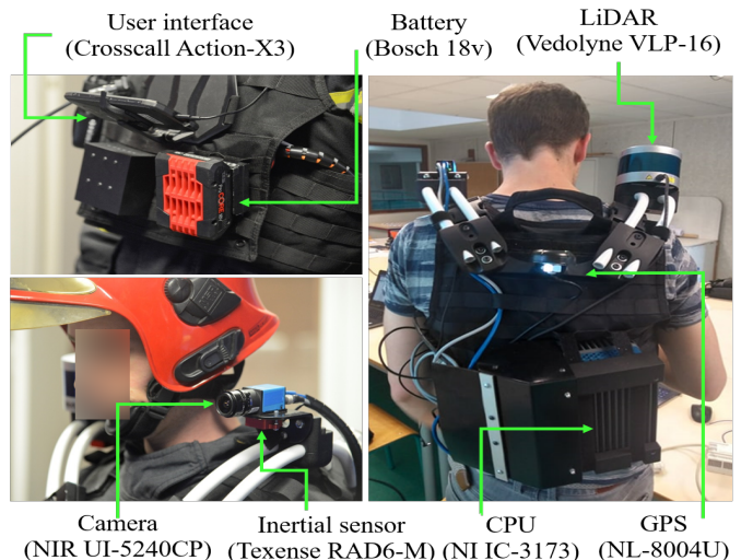
Fig. 2. Tactical waistcoat hardware configuration.
