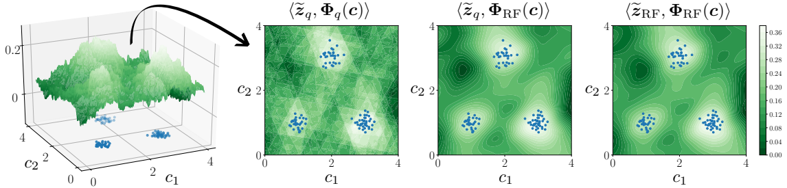
Fig. 13: Criterion \langle \tilde{\mathbf{z}}, \Phi(\mathbf{c}) \rangle versus centroid hypothesis \mathbf{c} = [c_1, c_2]^\top used by greedy parameter estimation algorithms in compressive clustering with k = 3 and a 2D dataset (in blue), with and without quantization of the sketch \tilde{\mathbf{z}} and/or feature map \Phi . The surface plot on the left highlights the irregularity of \mathbf{c} \mapsto \langle \tilde{\mathbf{z}}_q, \Phi_q(\mathbf{c}) \rangle .
