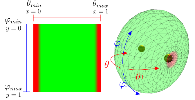
Figure 4: (x, y) texture mapping expressed in the Toric space (\theta, \phi) .
