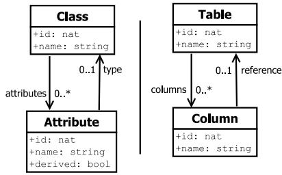
Figure 1: Minimal metamodelling for class diagrams (left), and relational schemas (right).
