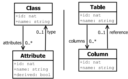
Figure 1: Minimal metamodels for class diagrams (left), and relational schemas (right).
