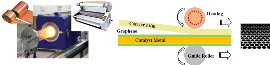
Fig. 8. Concept of transfer method after synthesis of graphene
