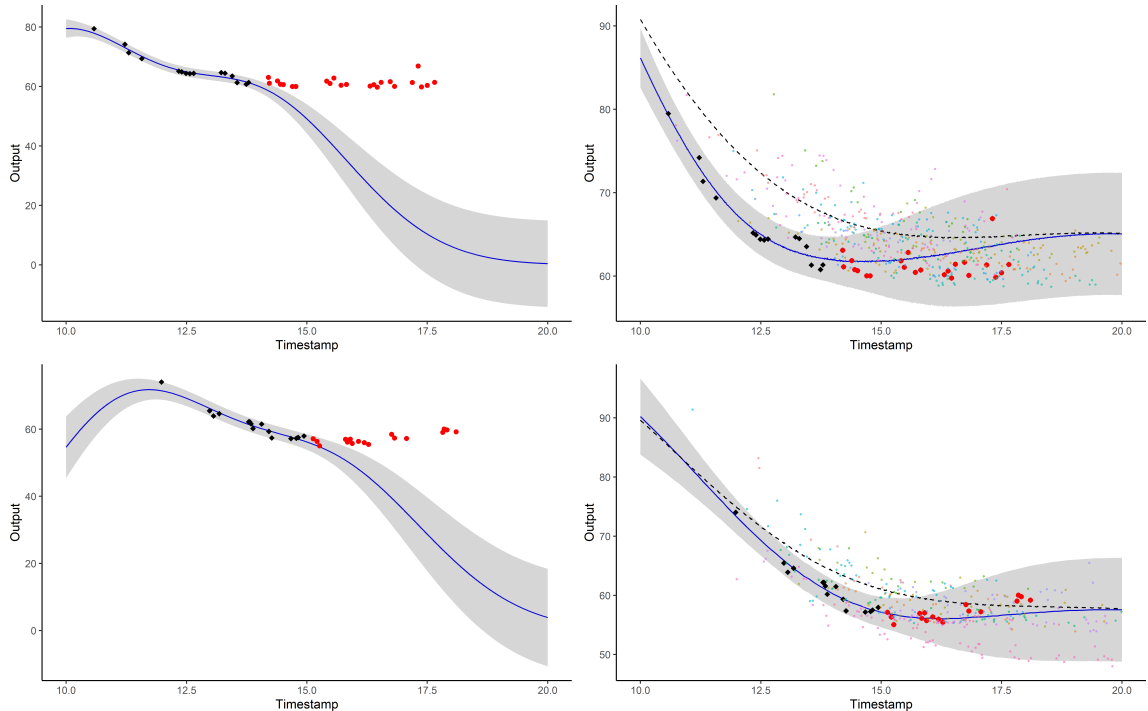
Figure 5: Prediction curves (blue) for a testing individual with associated 95% credible intervals (grey) for GP regression (left) and MAGMA (right), for both women (top) and men (bottom). The dashed lines represent the mean functions \hat{m}_0 , from the hyper-posterior p(\mu_0 | \{y_i\}_i) . Observed data points are in black, and testing data points are in red. The colourful backward points are observations from the training datasets, each colour corresponding to a different individual.
