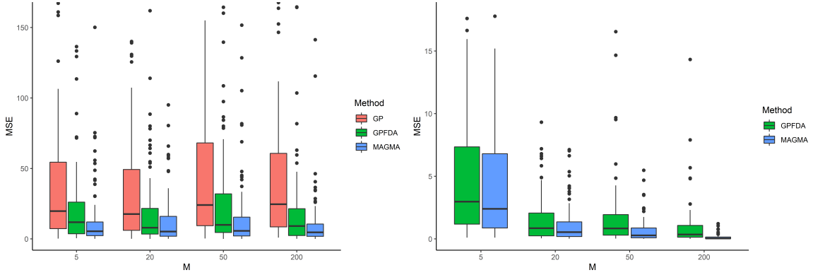
Figure 3: MSE with respect to the number M of training individuals (boxplots are displayed from 100 runs in each case). Left : prediction error on 10 testing points. Right : estimation error of the true mean process \mu_0 .
