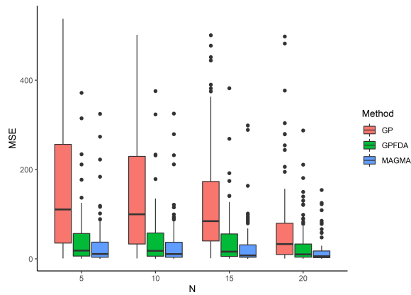
Figure 4: MSE prediction error on the 10 last testing points with respect to the increasing number N of observed timestamps, among the first 20 points (boxplots are displayed from 100 runs in each case).
