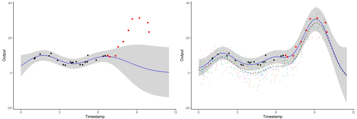
Figure 2: Prediction curves (blue) of a new individual with associated 95% credible intervals (grey) for GP regression (left) and MAGMA (right). The dashed line represents the mean function \hat{m}_0 , from the hyper-posterior p(\mu_0 \mid \{\mathbf{y}_i\}_i) . Observed data points are in black, and testing data points are in red. The colourful backward points are the observations from the training dataset, each colour corresponding to a different individual.
