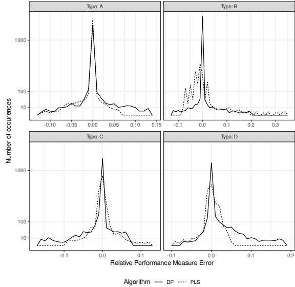
Figure 3: Absolute error between the relative performance measure of the predicted and real performance profiles.
