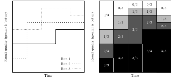
Figure 1: On the left the performance traces of three runs of an algorithm. On the right the corresponding performance profile for these runs.
