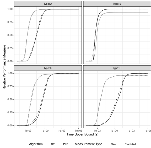
Figure 2: Relative performance measure for the “real” performance profiles (continuous lines) of testing instances of size n = 115 , and for the performance profile (discontinuous lines) predicted by our selection methodology.
