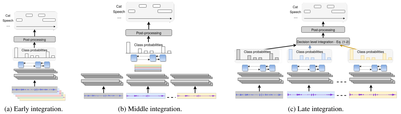
Figure 1: Integration between the SS and SED (gray waveform represents mixture, and colored waveforms represent separated sources).
