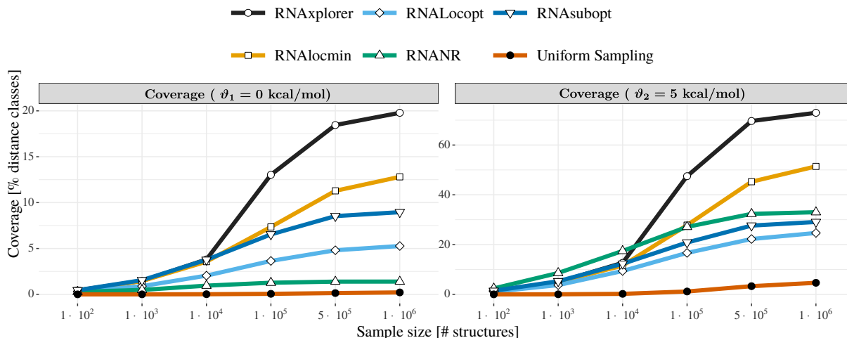
Figure 4: Distance class coverage as a function of sample size. Shown are the fractions of distance classes \mathcal{C}^{d_1, d_2} covered by at least one local minimum derived from the sample set that is energetically close to the respective \text{MFE}^{d_1, d_2} . The data averages over all 9 benchmark sequences, 10 independent runs per tool and margins \vartheta_1 = 0 kcal/mol (left plot), and \vartheta_2 = 5 kcal/mol (right plot).
