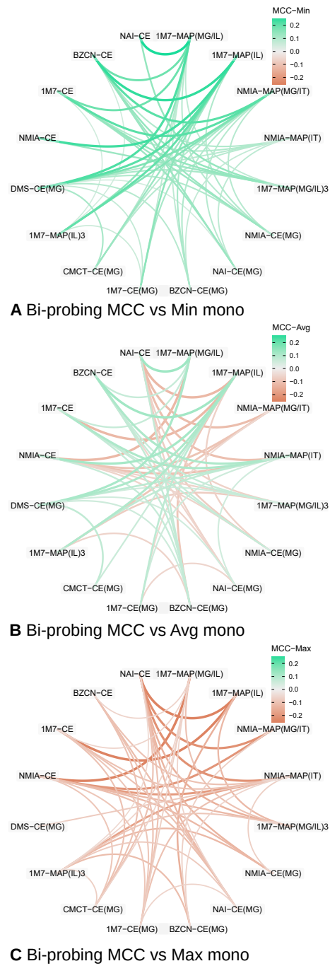
Figure 7: Shift in IPANEMAP predictive capacity (MCC) observed upon considering two conditions, compared to the worst ( A ), average ( B ) and best ( C ) predictions achieved for mono-probing conditions. Green and red edges indicate enhanced and degraded predictions respectively compared to the reference (Min, Max or Average of conditions). Thickness indicates absolute shift value (only values above 5% reported for readability).
