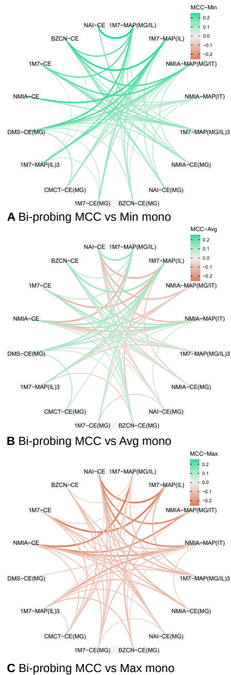
Figure 7: Shift in IPANEMAP predictive capacity (MCC) observed upon considering two conditions, compared to the worst (A), average (B) and best (C) predictions achieved for mono-probing conditions. Green and red edges indicate enhanced and degraded predictions respectively compared to the reference (Min, Max or Average of conditions). Thickness indicates absolute shift value (only values above 5% reported for readability).
