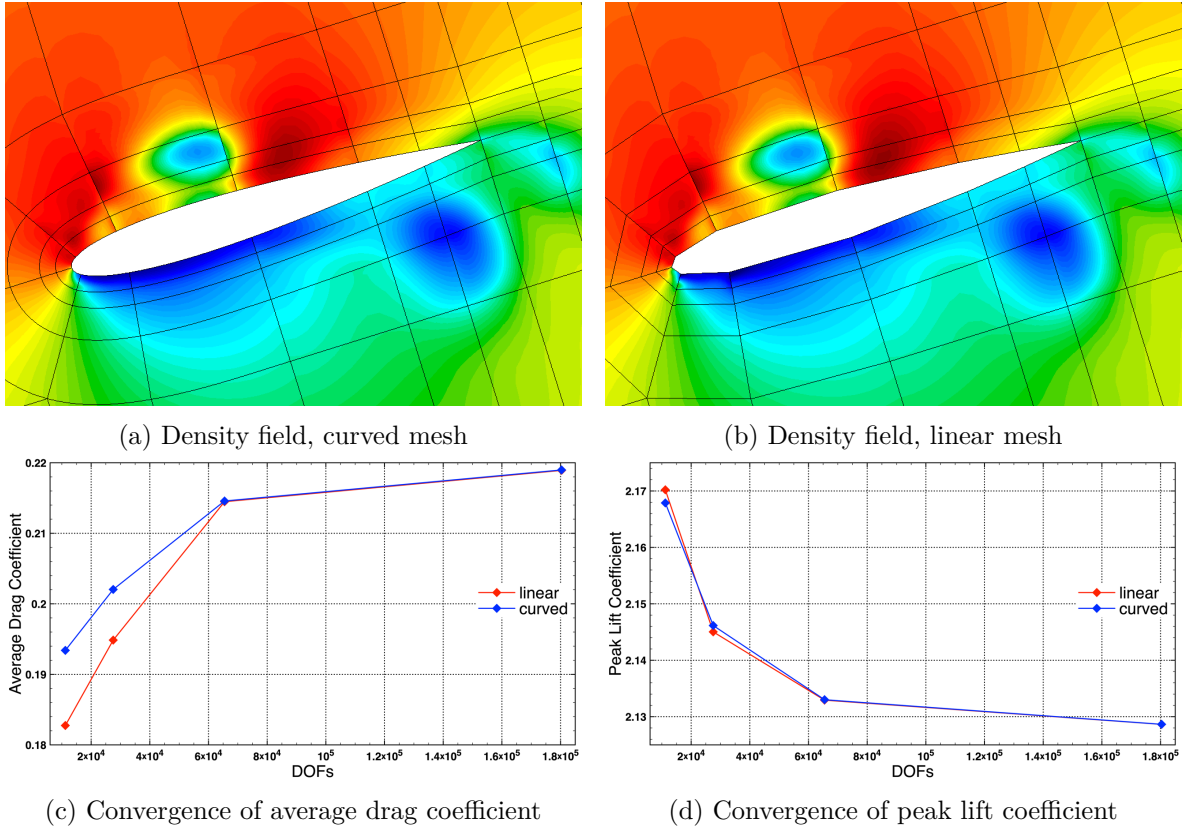
Figure 17: Influence of the geometry, laminar flow
