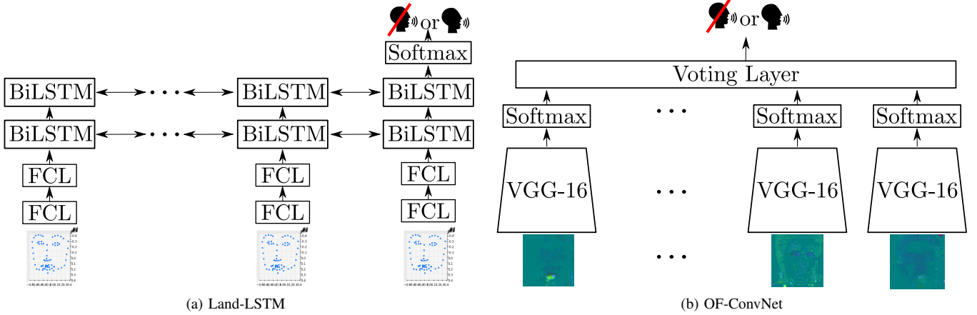
Fig. 1: Architectures of the two proposed models. Both networks take as input a sequence of frames and predict as output an activity label, speaking or silent .
