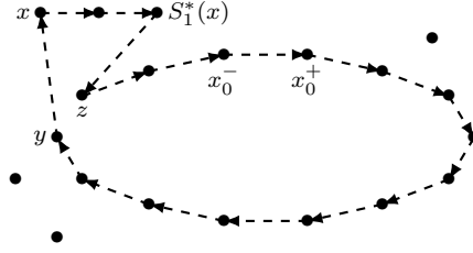
Figure 7: Inserting x in the S_1 -cycle, as in the second part of Algorithm 4, with one frequent type
