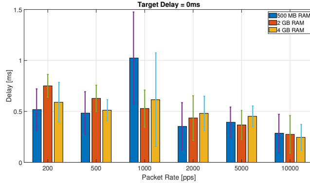
Fig. 5. Static Delay results with target value equal to 0 ms. Effect of RAM size variation.
