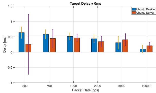
Fig. 7. Static Delay results with target value equal to 0 ms. Effect of Operating System variation.
