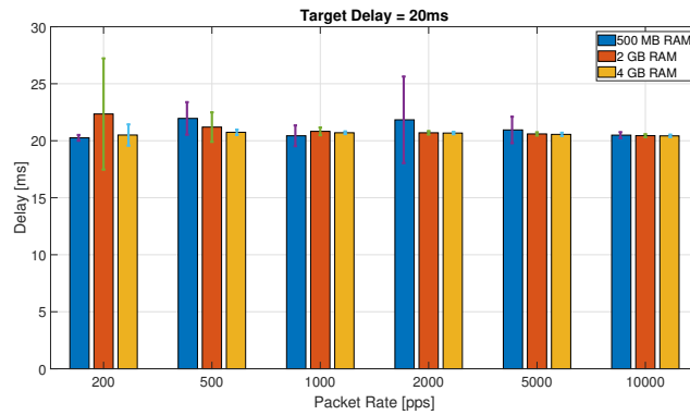
Fig. 6. Static Delay results with target value equal to 20 ms. Effect of RAM size number variation.
