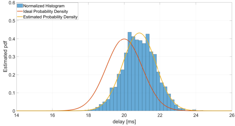
Fig. 10. Comparison of probability distributions: 2 GB RAM – 2 core CPU – Ubuntu Desktop OS
