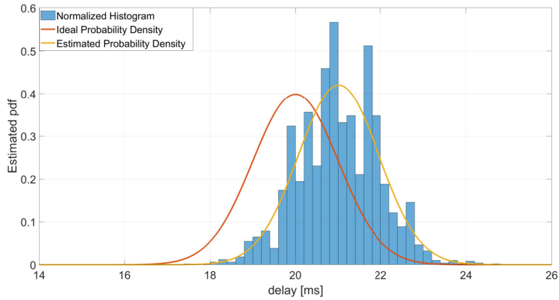
Fig. 9. Comparison of probability distributions: 500 MB RAM – 1 core CPU – Ubuntu Desktop OS
