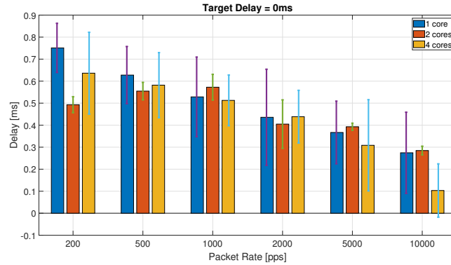
Fig. 3. Static Delay results with target value equal to 0 ms. Effect of CPU core number variation.
