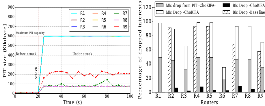
Fig. 4. PIT usage, base-line (solid lines) and ChoKIFA (dotted lines). Fig. 5. BI and MI drop, base-line and ChoKIFA.
