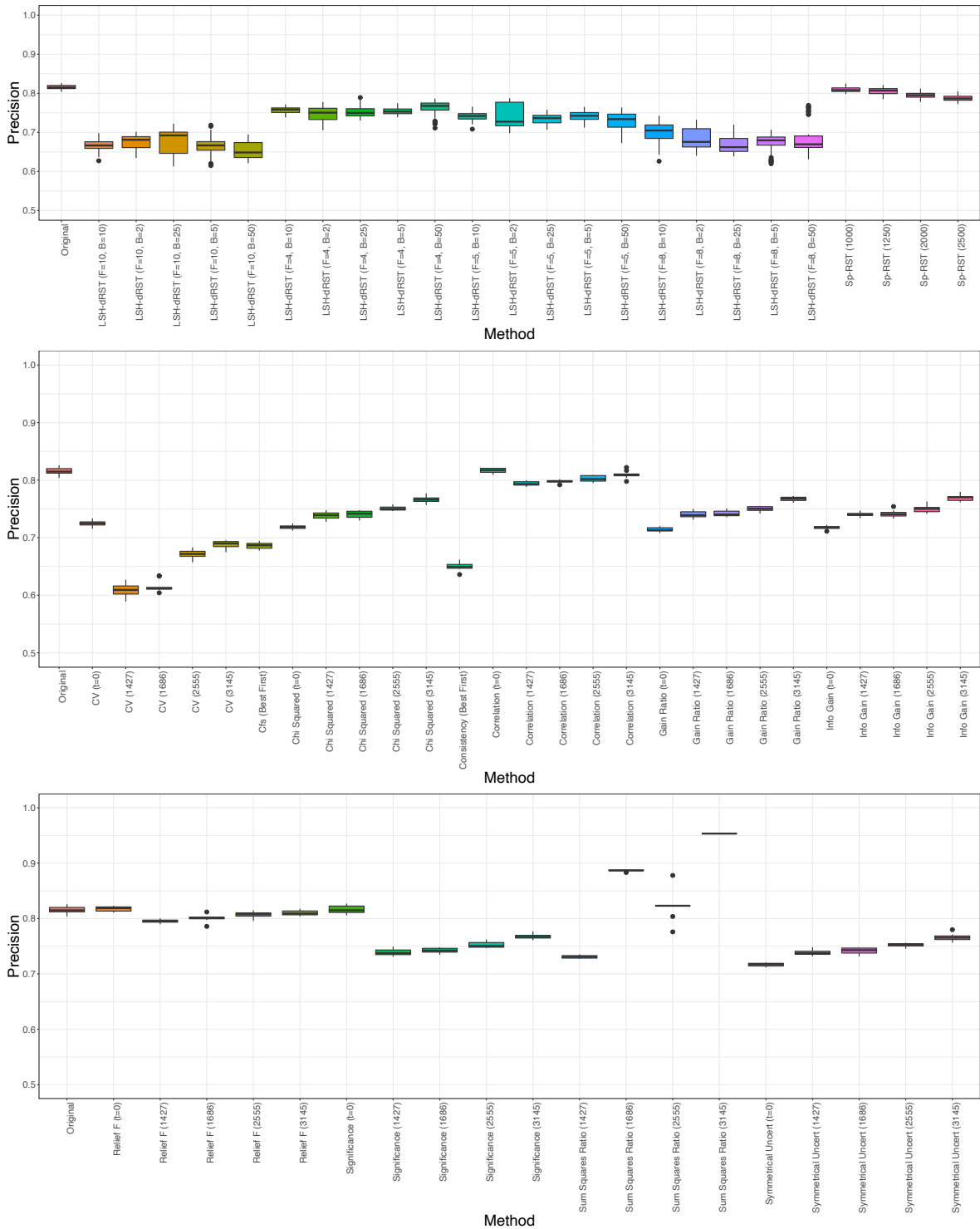
Figure 15. Random Forest: Precision for different parameters of LSH-dRST, Sp-RST and other feature selection techniques.
