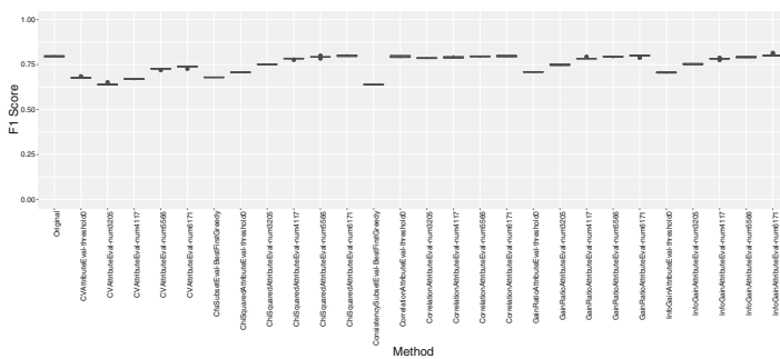
Fig. 17 Random forest classification results for other feature selection techniques (Part 1)
