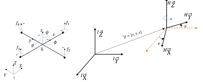
Fig. 1. Quadrotor coordinates and the horizon frame
