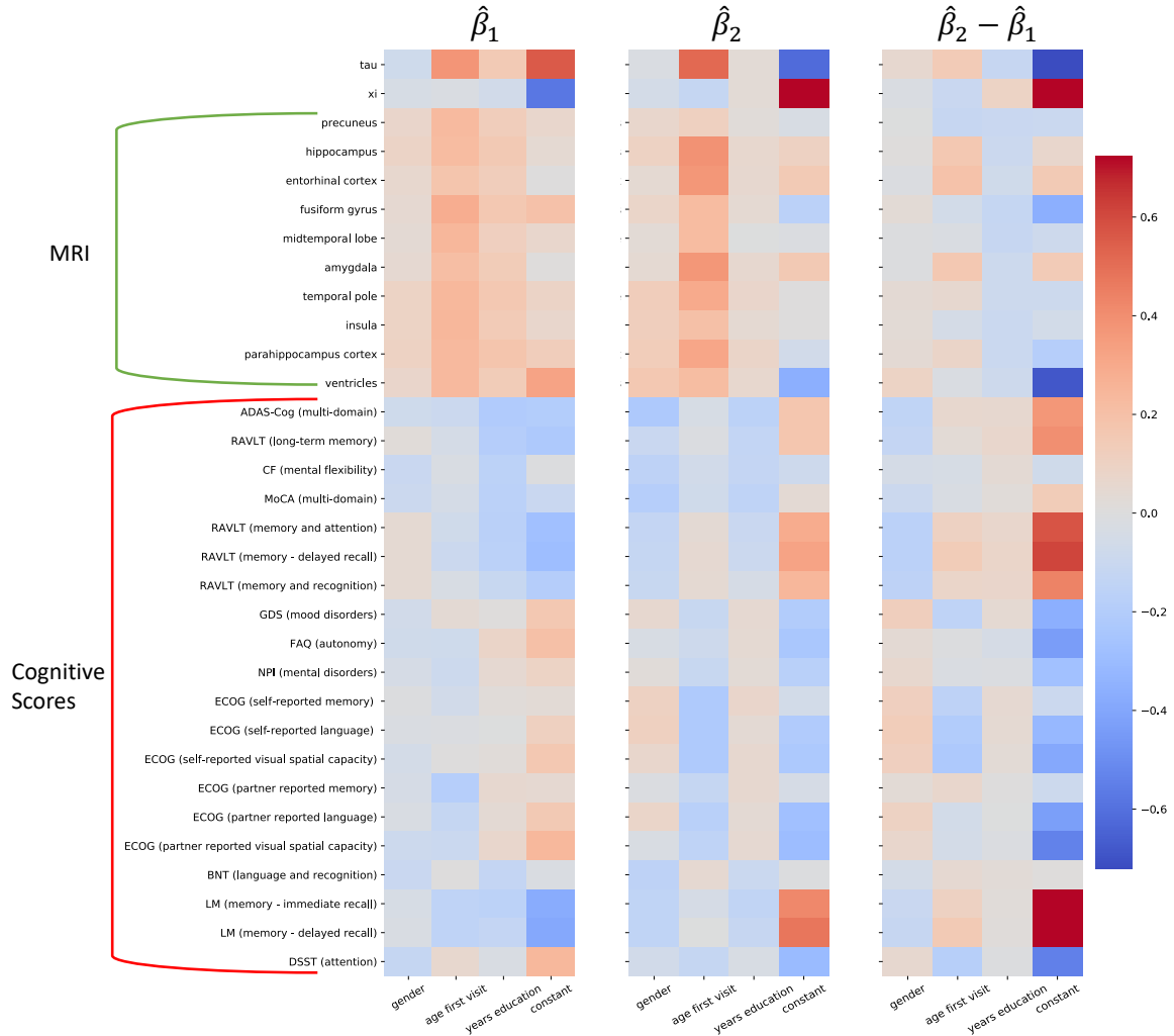
Fig. 7 Average of \hat{\beta}_k := -\hat{\Sigma}_k \hat{\Theta}_k^T over 10 bootstrap sampling of the data. For each bootstrapped dataset, \hat{\Sigma}_k and \hat{\Theta}_k are estimated with the C-EM. We make 3 of these C-EM runs, each starting from a different KMeans initialisation of the labels. This results in 10 \times 3 = 30 different estimates of \hat{\beta}_k to average over. (Left) \hat{\beta}_1 , the cluster k = 1 is always very correlated with the Control patients sub-population (less than 10% deviation). (Middle) \hat{\beta}_2 , the cluster k = 2 is likewise very correlated with the AD patients . In each figure, the last column is the constant coefficient. The largest inter-cluster differences are between the two constant terms. However there are some noticeable difference on the other regression coefficients as well. (Right) Average \hat{\beta}_2 - \hat{\beta}_1 over the 30 bootstrap runs of the C-EM. Here, the differences in intensity between AD ( k = 2 ) and Control ( k = 1 ) clusters are more explicit.
