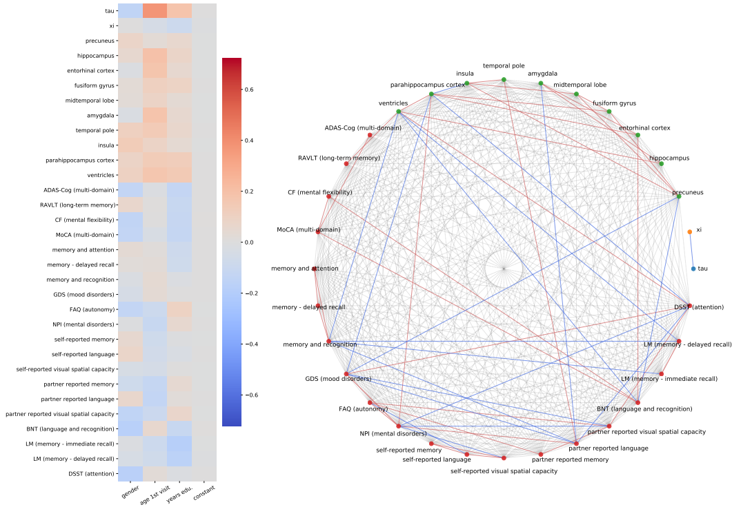
FIG 10. Parameters estimated with a simple CGGM on all data. (Left) \hat{\beta} = -\widehat{\Sigma}\widehat{\Theta} . (Right) Conditional correlations graph.
