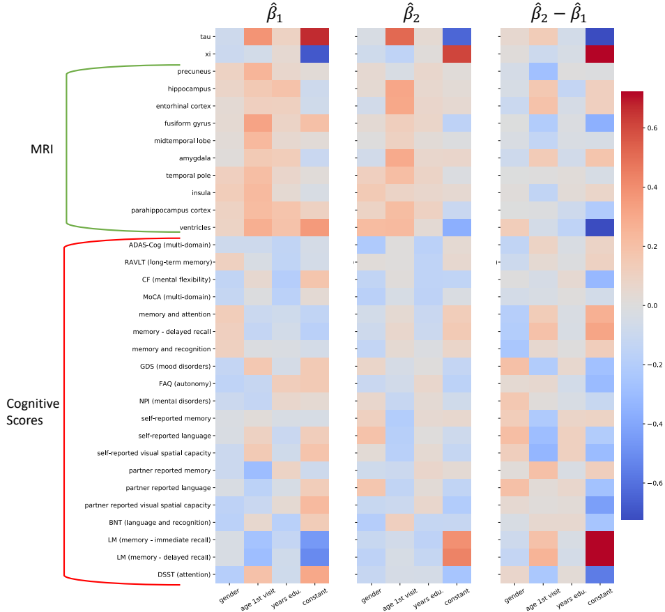
FIG 8. Oracle MLE \hat{\beta}_k := -\hat{\Sigma}_k \hat{\Theta}_k^T estimated with the knowledge of the real labels (supervised estimation). A comparison with Fig 7 shows that the C-EM properly recovered these structures. (Left) \hat{\beta}_1 , MLE of the Control patients sub-population. (Middle) \hat{\beta}_2 , MLE of the AD patients . (Right) \hat{\beta}_2 - \hat{\beta}_1 , their difference in intensity .
