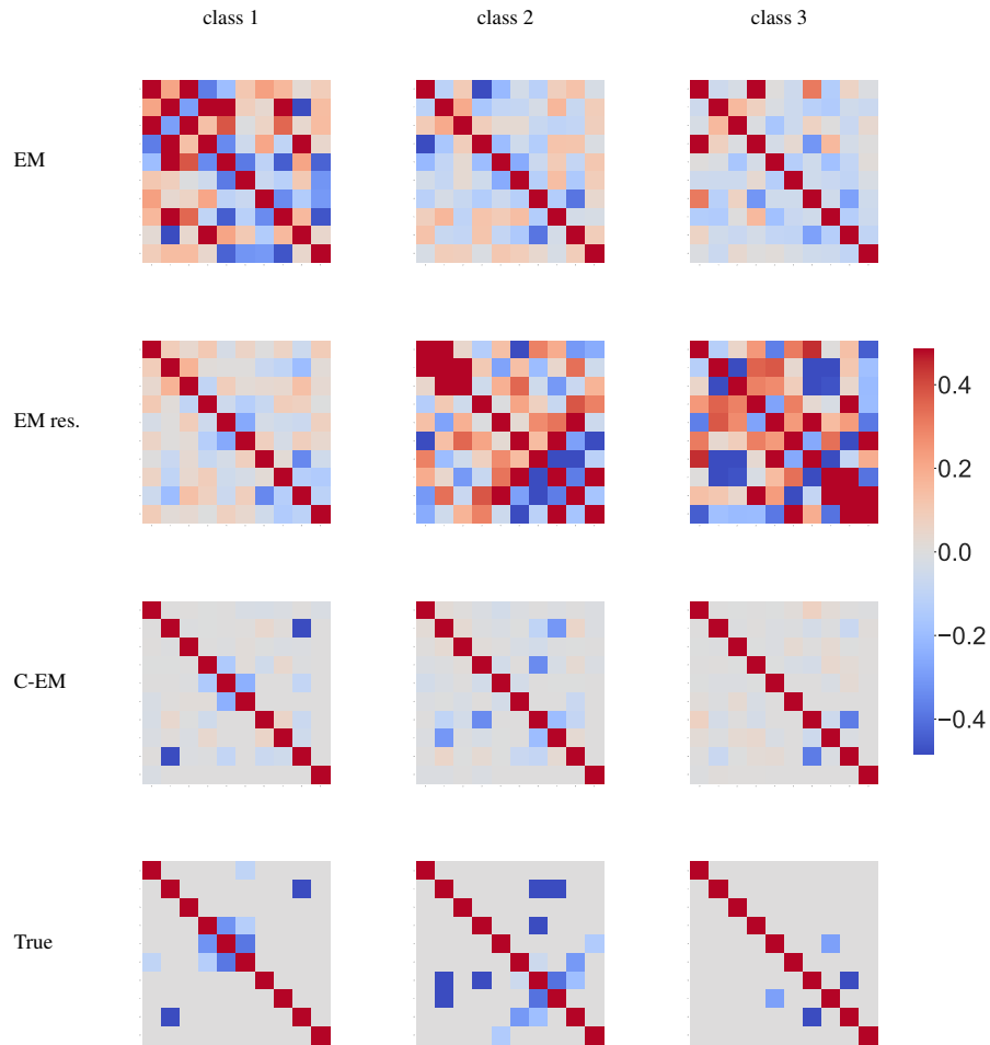
FIG 5. Comparison between the several estimated and the true conditional correlation matrices for each sub-population. The three columns of figures correspond to the three sub-populations. The first two rows of figures are the matrices estimated by the two Mixture of GGM methods, with and without residualisation with the co-features. The third row of figures correspond to the matrices estimated by the Mixture of CGGM. The final row displays the real conditional correlation matrices. Unlike the two GGM-based methods, the Mixture of CGGM recovers correct edges with very few False Positives.
