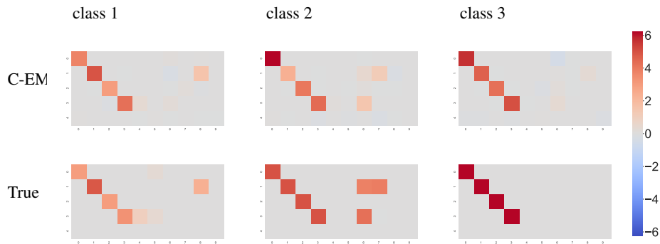
FIG 6. Reconstruction of the \Theta_k by the EM on the Mixture of CGGM. The three columns of figures correspond to the three sub-populations. Almost all the edges are right, with no False Positive and almost no False Negative. Moreover, the intensities are also mostly correct.
