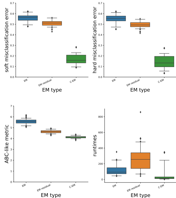
Fig. 4 Empirical distribution of several performance metrics measured over many simulations. The sample is made of 20 simulations with 5 different initialisations each. Three methods are compared. The EM and EM residual algorithms estimate a Mixture of GGM. The C-EM algorithm estimates a Mixture of CGGM. The C-EM is much better performing and faster. (Upper left) Soft mis-classification error |\mathbb{1}_{z_i=k} - \hat{\mathbb{P}}(z_i = k)| . (Upper right) Hard mis-classification error |\mathbb{1}_{z_i=k} - \mathbb{1}_{\hat{z}_i=k}| . (Bottom left) ABC-like metric. (Bottom right) Run time.
