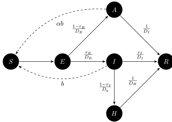
Figure 6: SEIRAH model representation – adapted from [52]
