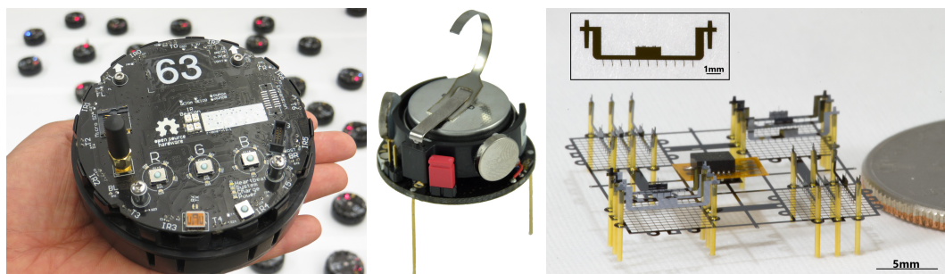
Figure 1: Robots used in swarm robotics come in different shapes and sizes: the dm -scale r-one [1] (left), the cm -scale kilobot [2] (center), the mm -scale ionocraft [3] (right).
