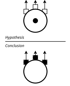
Figure 6: Rule \text{Leave}_\pi .
