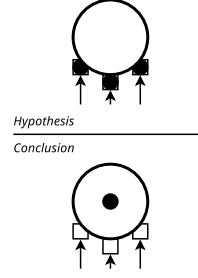
Figure 5: Rule \text{Reach}_\pi .
