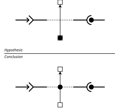
Figure 7: Rule \text{Fire}_\theta .
