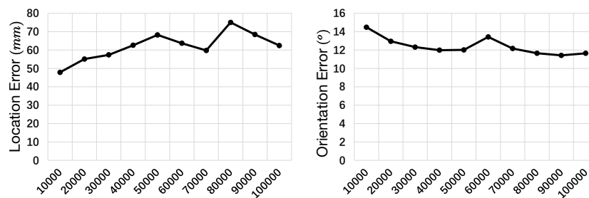
Figure 12. Estimated camera location (mm) and orientation ( ^{\circ} ) errors using different \beta values (x axis). \beta = 40,000 was finally selected for our experiments.
